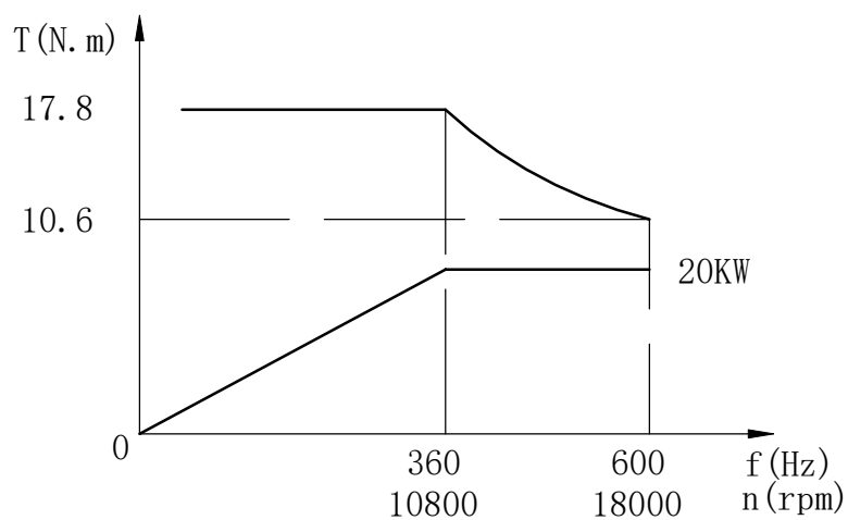
Torque/P.f Curve
