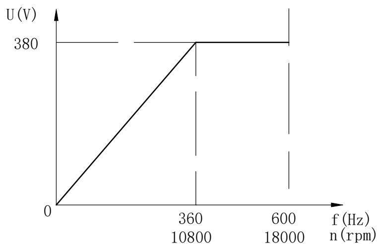
U.f Curve
