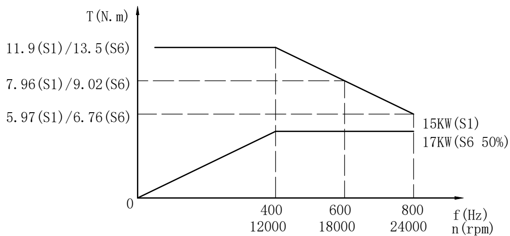
Torque/P. f Curve
