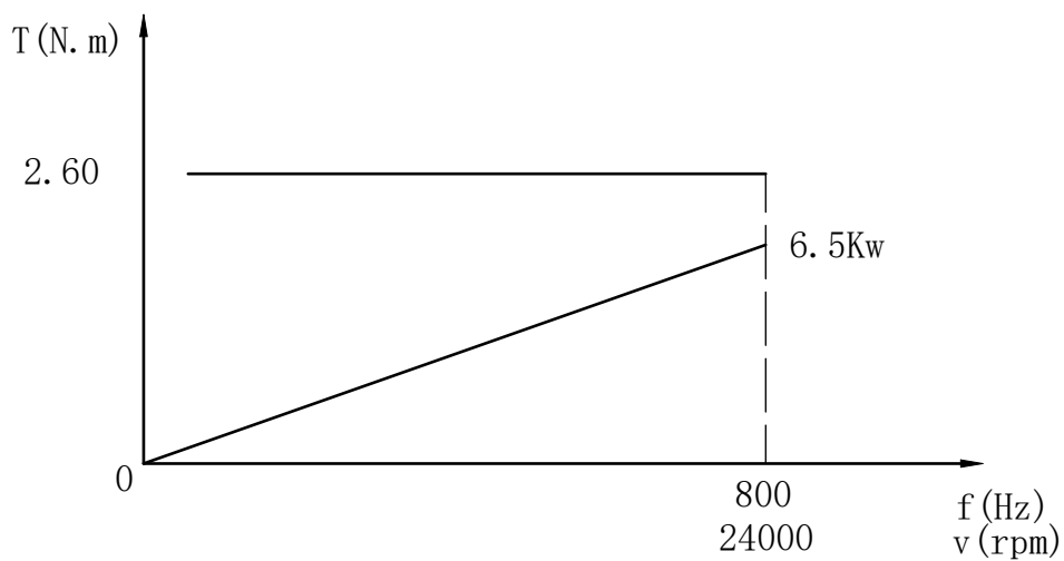
Torque/P. f Curve
