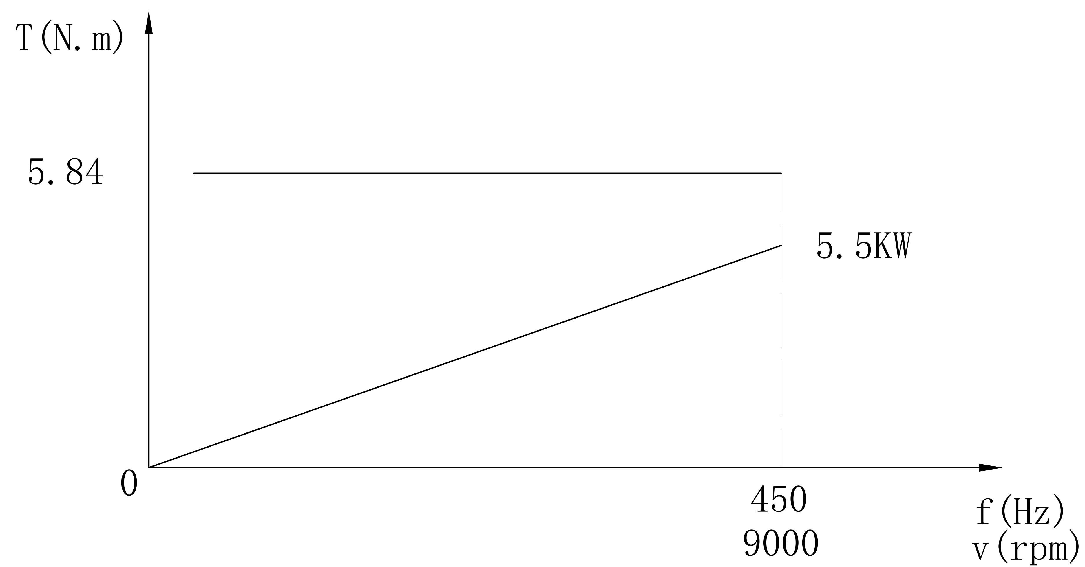
Torque/P. f Curve
