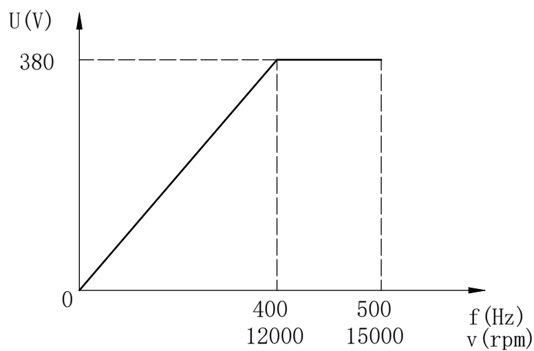
U.f Curve
