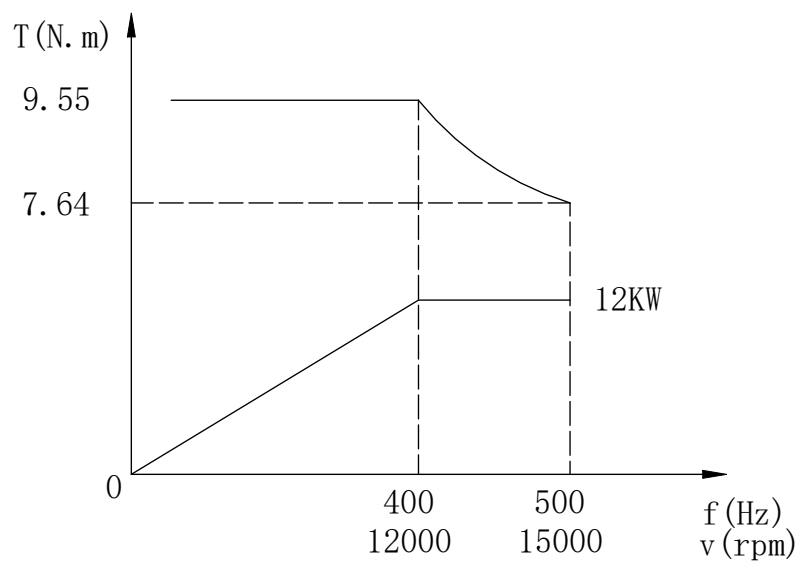
Torque/P.f Curve
