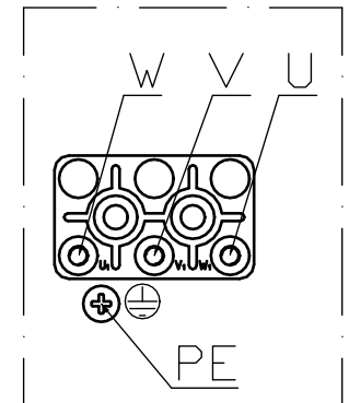
Wiring illustration
