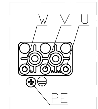
Wiring illustration
