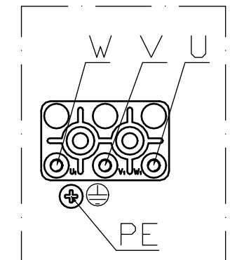
Wiring illustration
