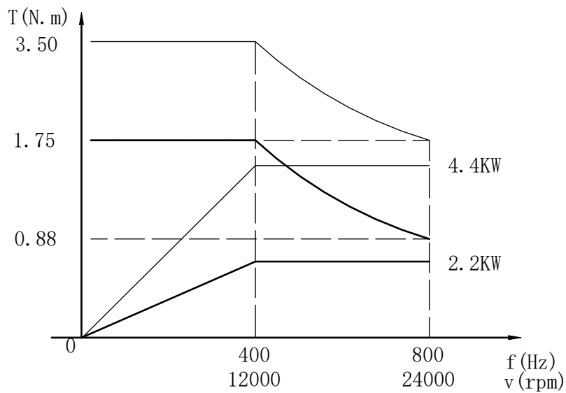
Torque/P. f Curve
