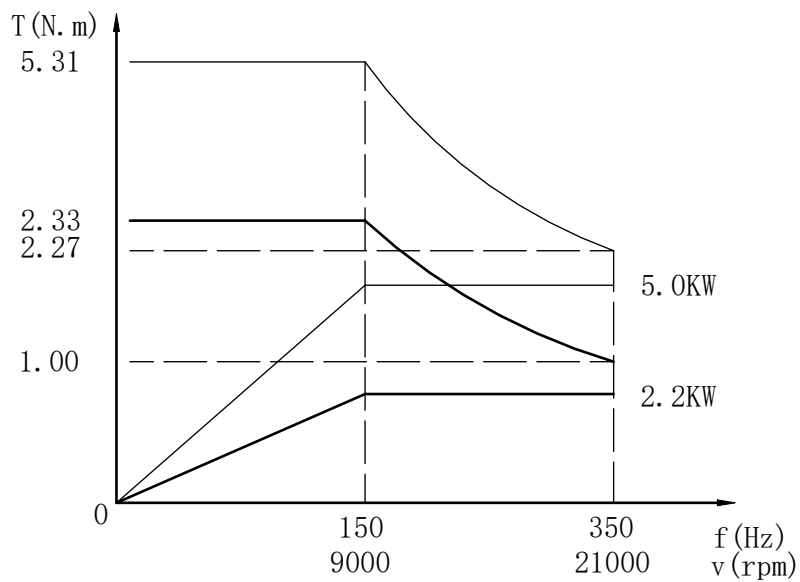
Torque/P. f Curve
