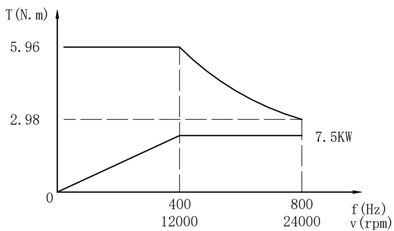
Torque/P. f Curve
