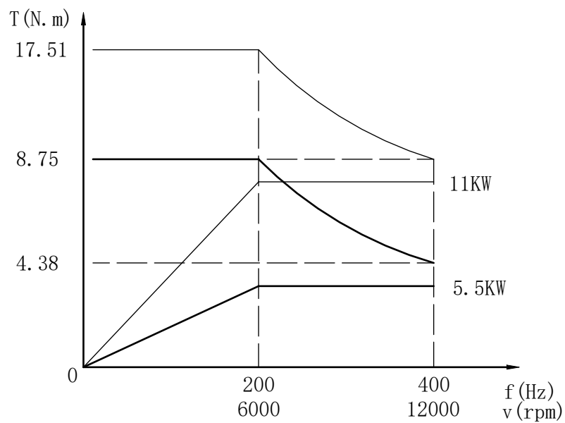
Torque/P. f Curve
