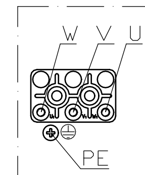
Wiring illustration
