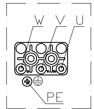
Wiring illustration
