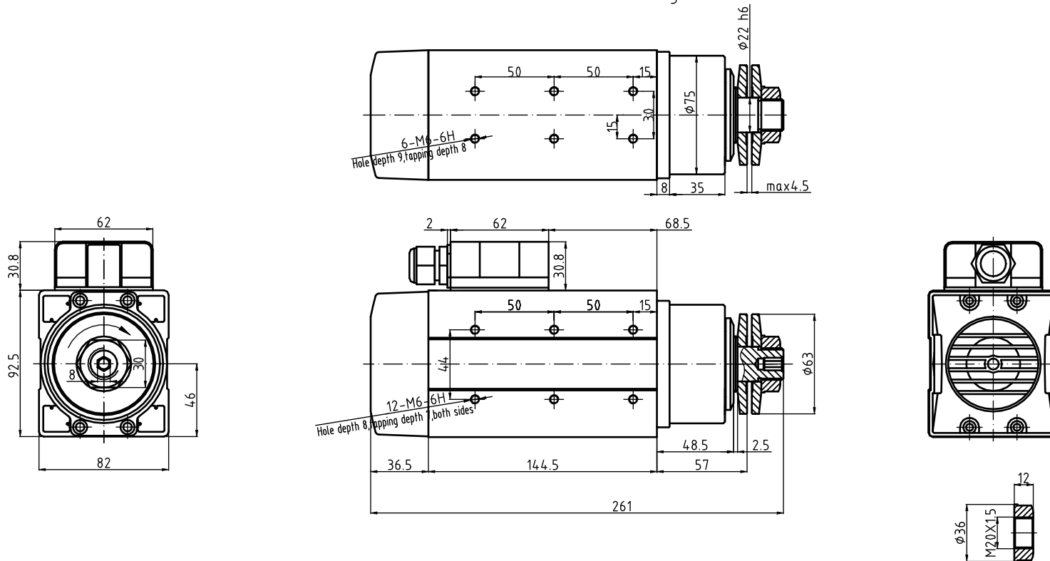
GDF46-12Z/1.5 220V/380V Profile drawing
