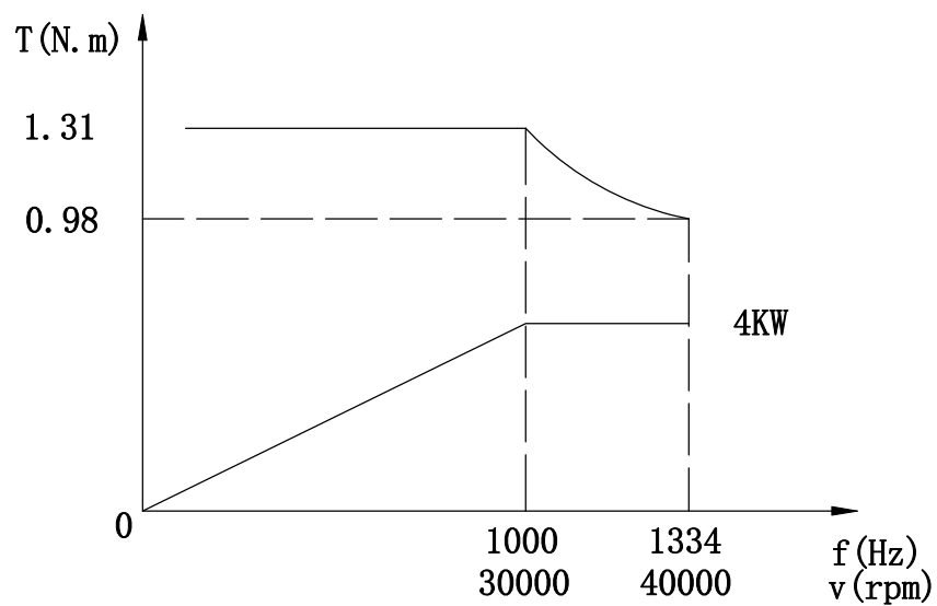
Torque/P.f Curve
