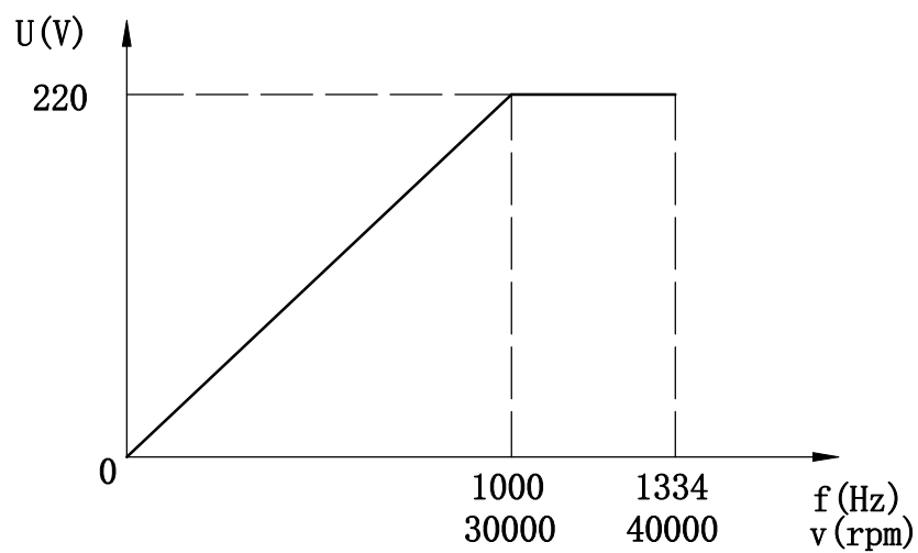
U.f Curve
